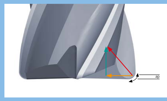
Toric tool
